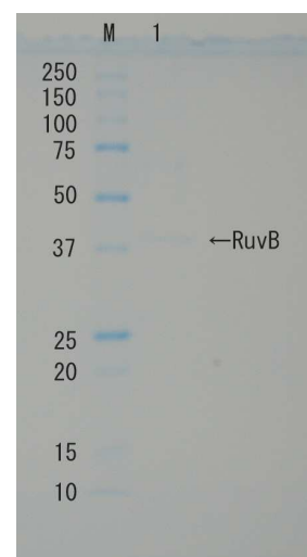
Fig. 1 Polyacrylamide gel electrophoresis of RuvB protein.
